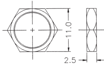
P/N RFA7-02 HEX NUT
