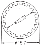
P/N RFA8-01 WASHER
