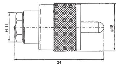
NP707CU-XNGD50 ROTATING NIPPLE MALE TO UHF MALE
