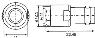
NP711CU-XNGD50 ROTATING NIPPLE MALE TO BNC FEMALE
