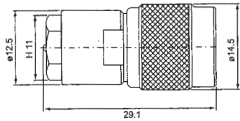
NP703CU-XNGD50 ROTATING NIPPLE MALE TO TNC MALE
