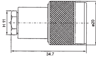
NP698CU-XNGD50 ROTATING NIPPLE MALE TO N MALE
