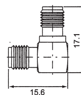
SA815CU-X*GT50 SMA DOUBLE FEMALE RIGHT ANGLE TYPE
