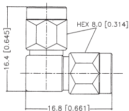
SA770CU-X*GT50 SMA DOUBLE MALE RIGHT ANGLE TYPE
