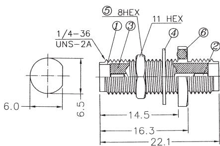
SA828CU-XGGT50 SMA DOUBLE FEMALE BULKHEAD TYPE
