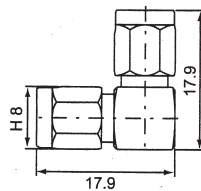
SA814CU-X*GT50 SMA DOUBLE MALE RIGHT ANGLE TYPE
