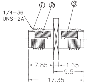
SA827CU-XGGT50 SMA DOUBLE FEMALE PANEL MOUNT TYPE
