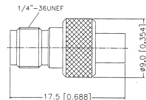
SA816CU-X*GT50 SMA FEMALE TO MCX FEMALE
