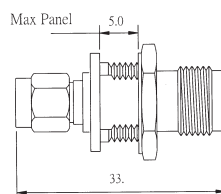
SA812CU-X*GT50 SMA MALE TO TNC FEMALE BULKHEAD TYPE
