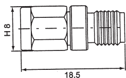
SA813CU-X*GT50 SMA MALE TO SMA FEMALE
