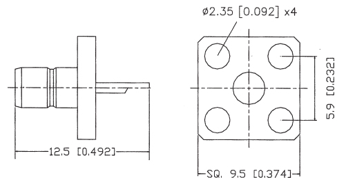
SB321CU-XGGT** SMB JACK PANEL MOUNT WITH 4 HOLE FLANGES PART NO.: SB321CU-XGGT50 SB321CU-XGGT75
