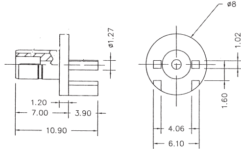
SB358CU-XGGT** SMB JACK STRAIGHT PCB MOUNT TYPE
