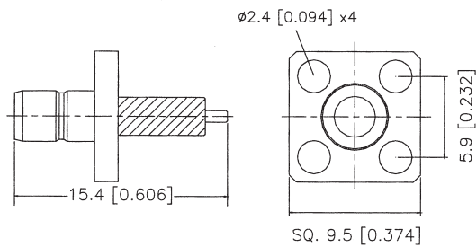
SB320CU-XGGT50 SMB JACK 4 HOLE FALNGE WITH EXPOSED TEFLON PANEL MOUNT TYPE
