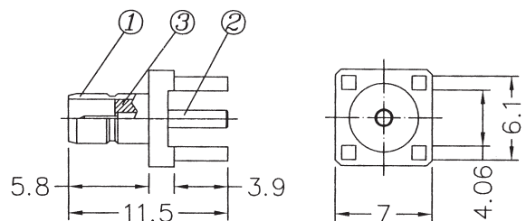
SB359CU-XGGT** SMB JACK WITH 4 LEGS PCB MOUNT TYPE
