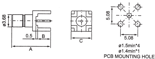
SB330CU-XGGT** SB331CU-XGGT** SMB JACK STRAIGHT PCB MOUNT TYPE
