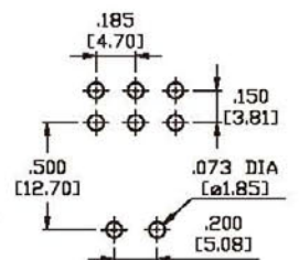
P.C. MOUNTING
