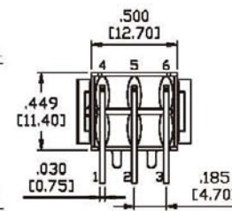
P.C. MOUNTING
