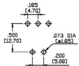
P.C. MOUNTING
