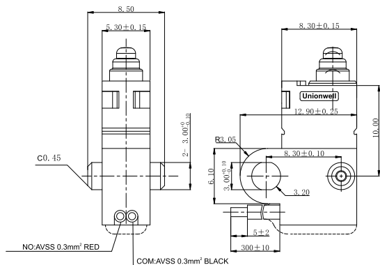
C-Type Waterproof Cover (Build-in Resistance) Wires Lead to Left
