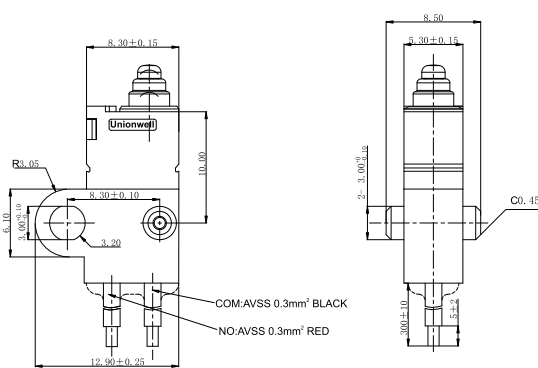
C-Type Waterproof Cover (Build-in Resistance) Wires Lead to Bottom
