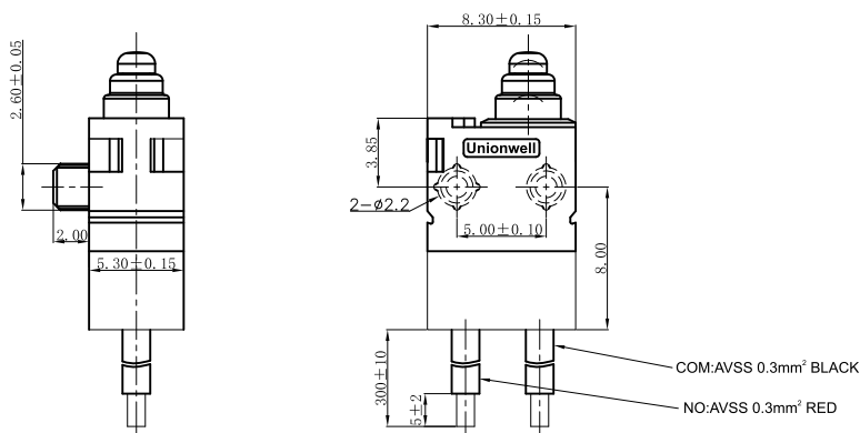
A-Type Waterproof Cover Wires Lead to Bottom
