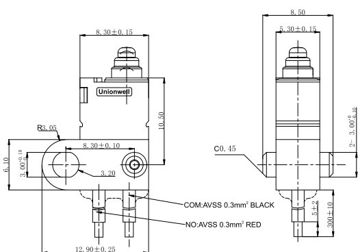
B-Type Waterproof Cover Wires Lead to Bottom
