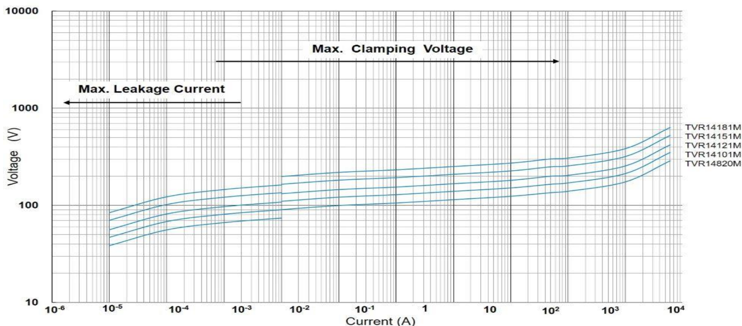
Max. Leakage Current and Max. Clamping Voltage Curves (TVR14820M to TVR14181M)
