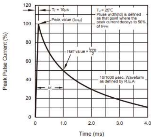
Fig.3 - Pulse Waveform
