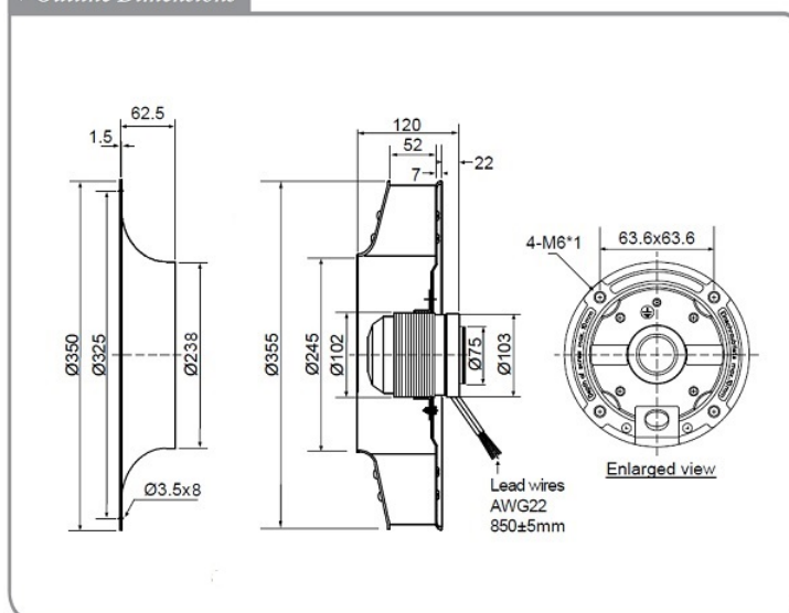
Inlet nozzle/Duct ring DR355SN
