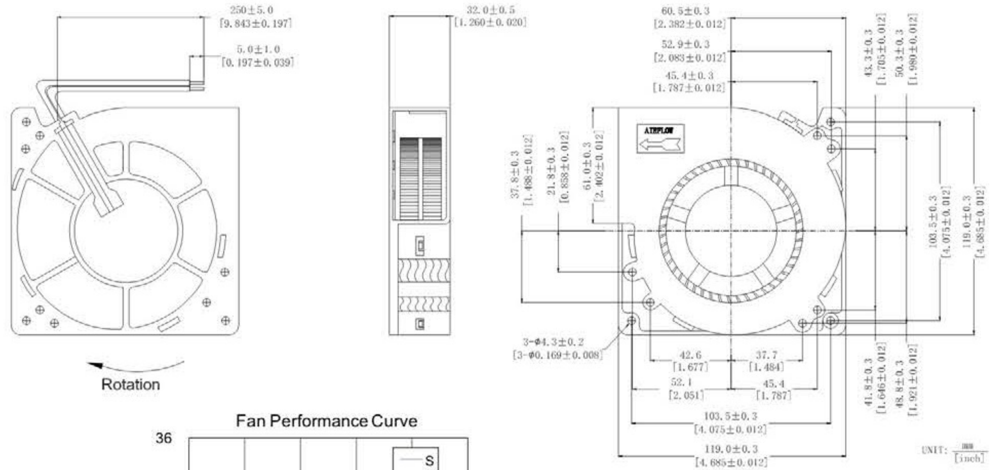
DIMENSIONS DRAWING
