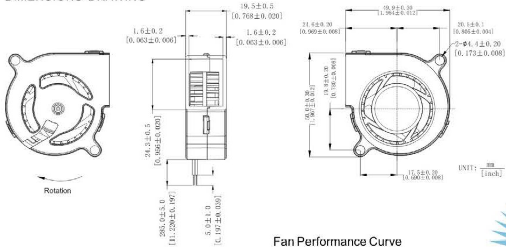
DIMENSIONS DRAWING
