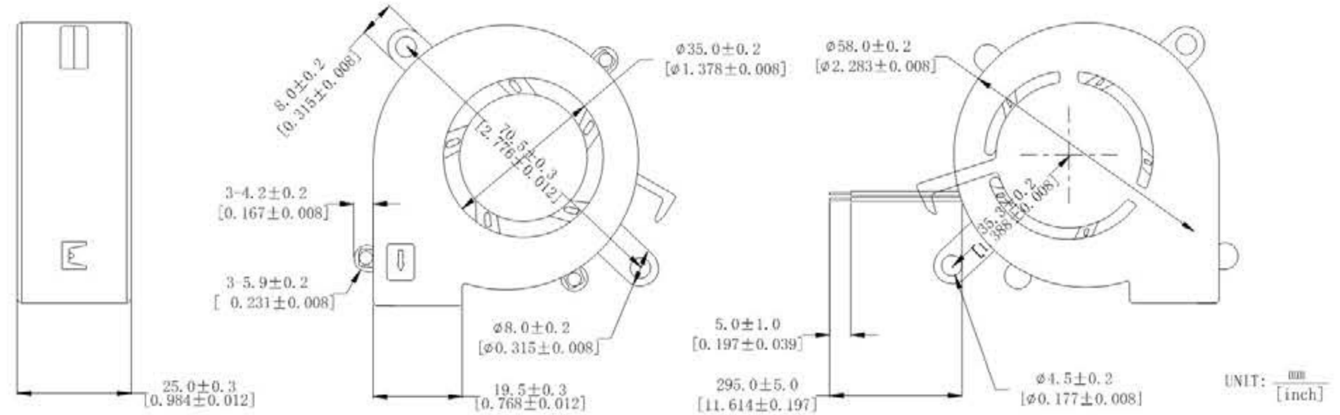
DIMENSIONS DRAWING
