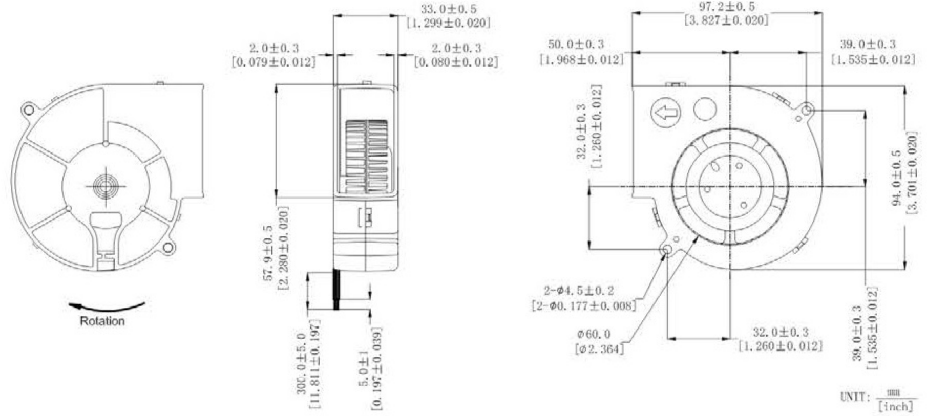
DIMENSIONS DRAWING
