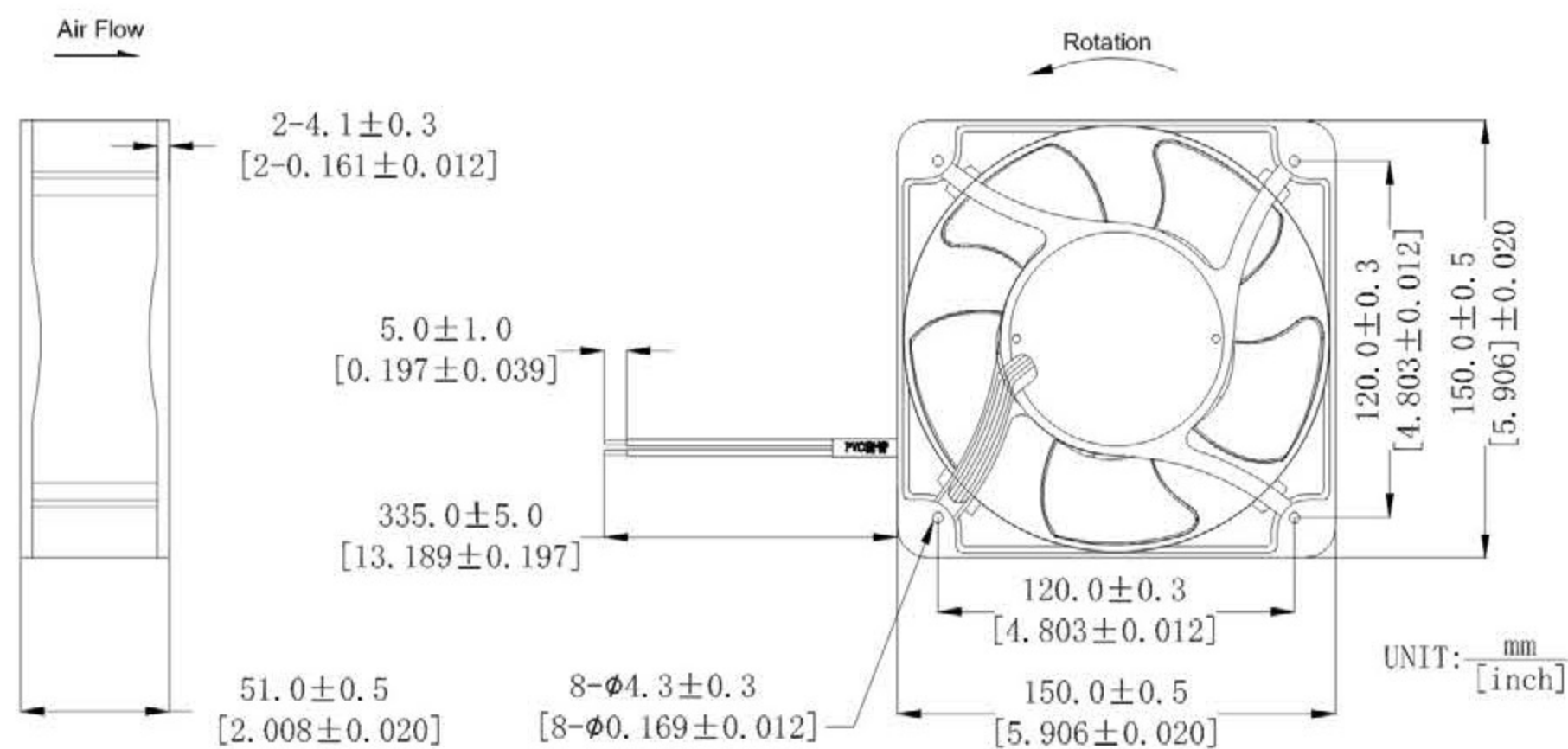
DIMENSIONS DRAWING
