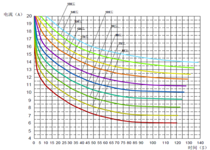
Current vs. Tripping time
