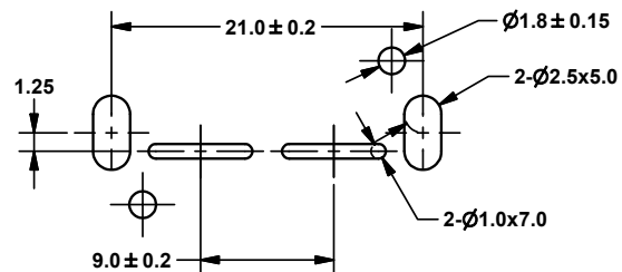
MOUNTING HOLES
