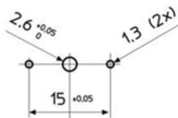
Mounting holes
