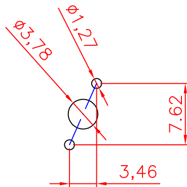
mounting pattern
