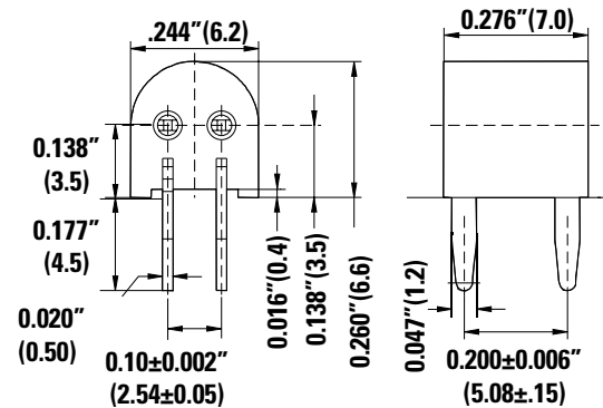
Circuit Board Mounting Detail
