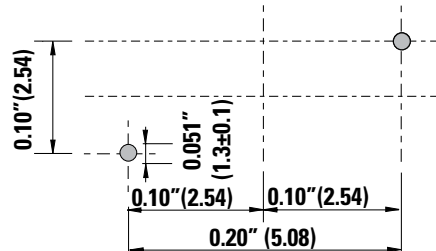
Circuit Board Mounting Detail
