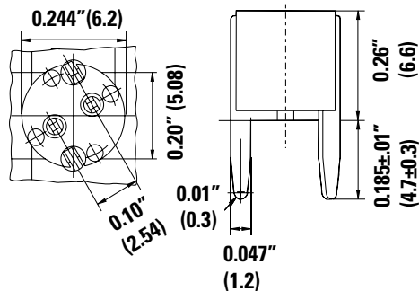
Circuit Board Mounting Detail
