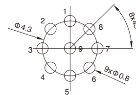
9Pins male
