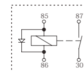
With diode
