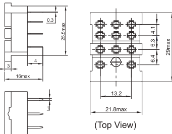
Outline dimensions (Unit: mm)
