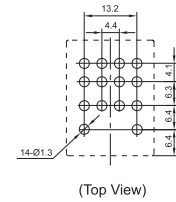
PCB layout
