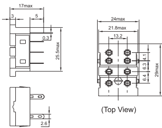
Outline dimensions (Unit: mm)
